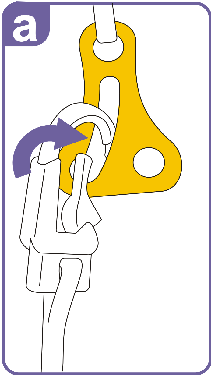
Clip the carabiner into the long opening of the TWEEZLE 8
